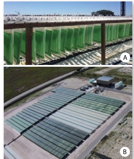
▲ Figure 7.6: Photobioreactor farm established at Algenol, Ft. Myers, FL, USA, (A) hanging bags designed to collect the headspace, (B) large-scale integrated algae-ethanol-producing farm
